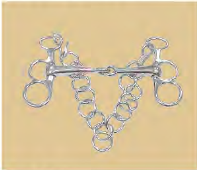
NO.3247 DRIVING BIT stainless steel, solid mouth Cheek:11cm Thickness:17mm 12.5cm(5") 13.5cm(5-1/4") 14.5cm(5-3/4") 25/Box
