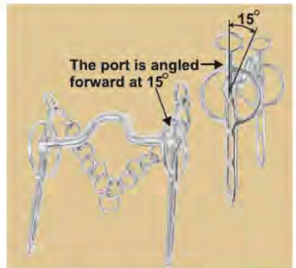
NO.3039 LIVERPOOL Fixed 15 Stainless steel Cheek:18.5cm Thickness:12mm 13.5cm(5-1/4") 14.5cm(5-3/4") 25/Box
