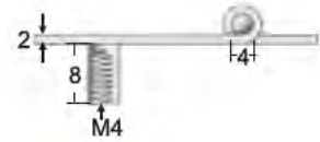
HINGE WITH THREAD SHANKS M4 stamped AISI 304 , buff polished ITEM NO. Thickness Weight/g 006150 2mm 44
