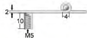
HINGE WITH THREAD SHANKS M5 stamped AISI 304 , buff polished ITEM NO. Thickness Weight/g 006154 2mm 53
